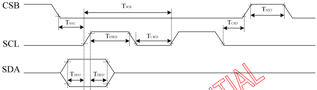
Figure 13.4: Serial interface characteristics
