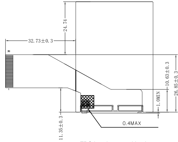
FPC bend on panel back
